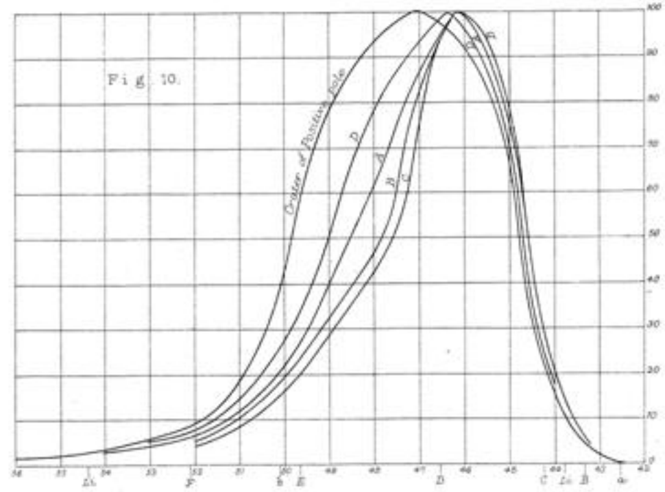
Fig. 10. Curve A is Incandescence lamp 102 Watts. Curve B is Incandescence lamp 143 Watts. Curve C is Incandescence lamp 266 Watts. Curve D gas flame.
